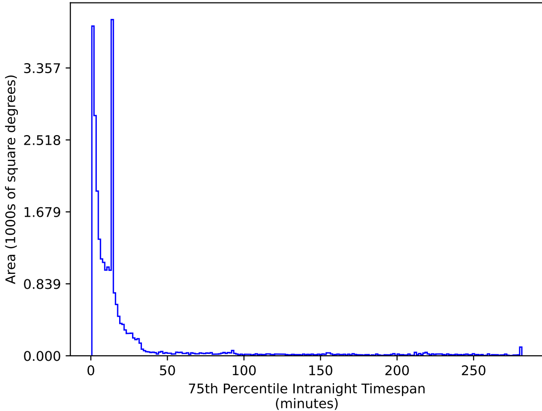
baseline_v3.2_10yrs All sky r band: 75th Percentile Intranight Timespan
