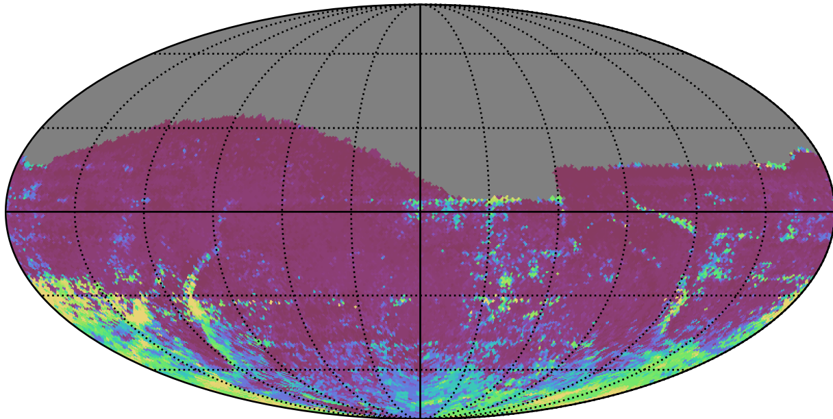
baseline_v3.2_10yrs All sky i band: 75th Percentile Intranight Timespan
