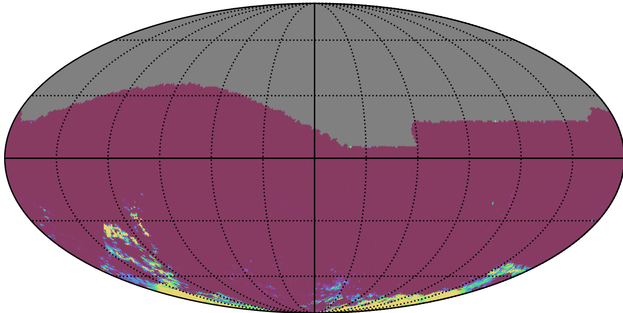
baseline_v3.2_10yrs All sky gr bands: 75th Percentile Intranight Timespan
