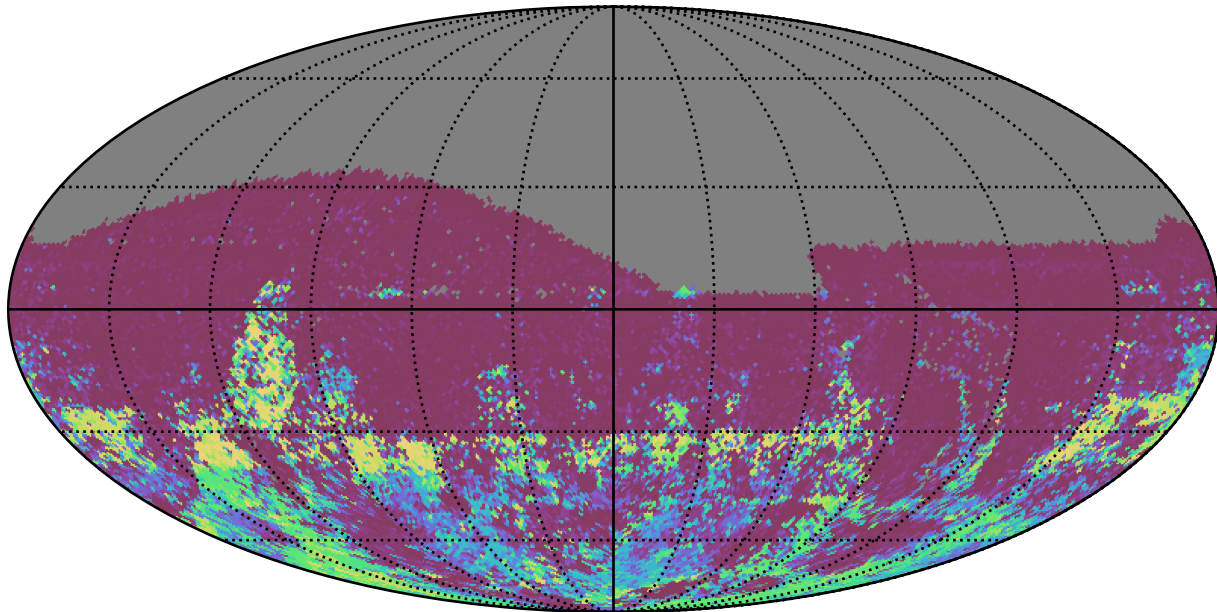
baseline_v3.2_10yrs All sky g band: 75th Percentile Intranight Timespan
