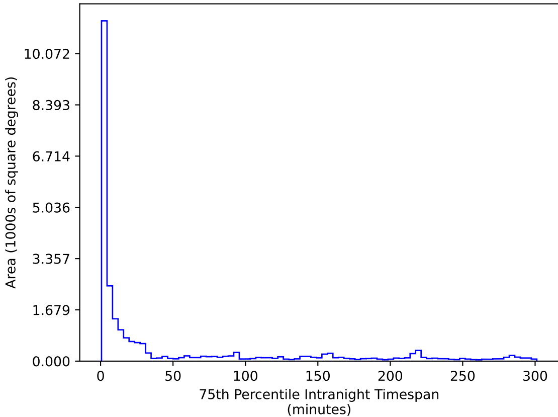
baseline_v3.2_10yrs All sky g band: 75th Percentile Intranight Timespan
