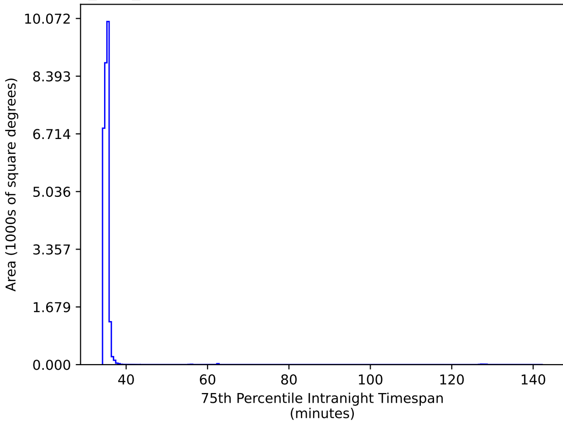
baseline_v3.2_10yrs All sky all bands: 75th Percentile Intranight Timespan
