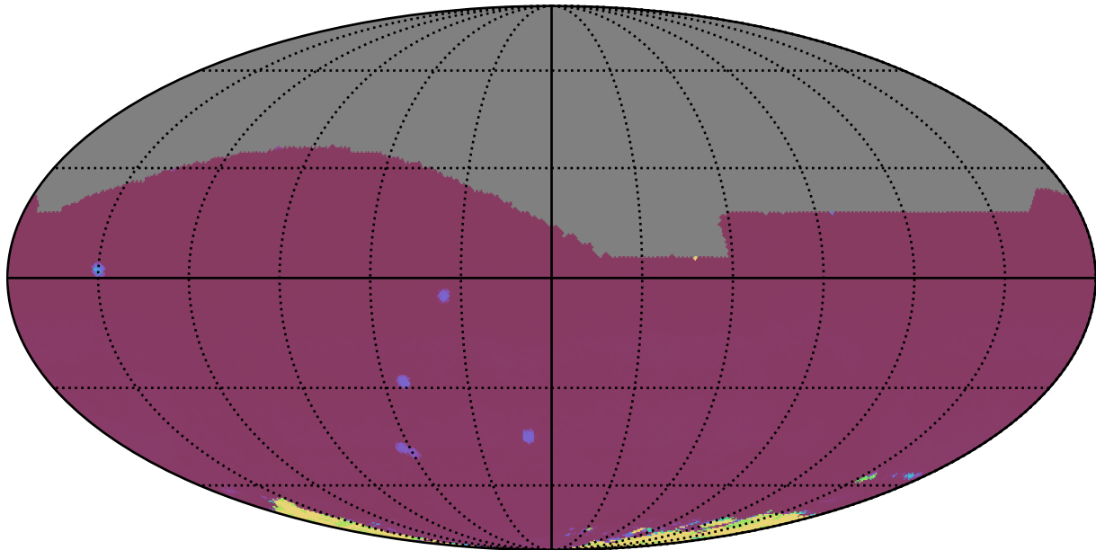
baseline_v3.2_10yrs All sky: 75th Percentile Intranight Timespan
