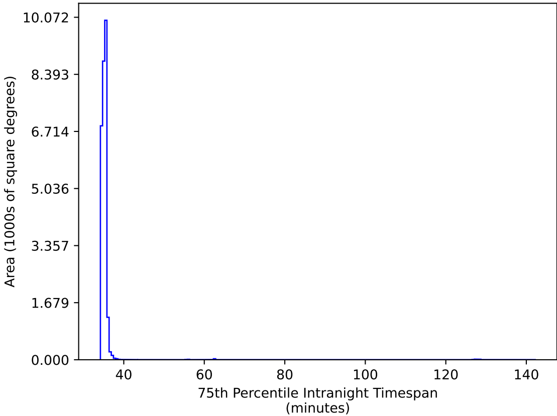
baseline_v3.2_10yrs All sky: 75th Percentile Intranight Timespan
