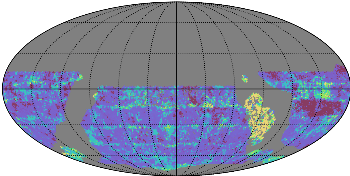
baseline_v3.2_10yrs WFD y band: 20thPercentile Inter-Night Gap
