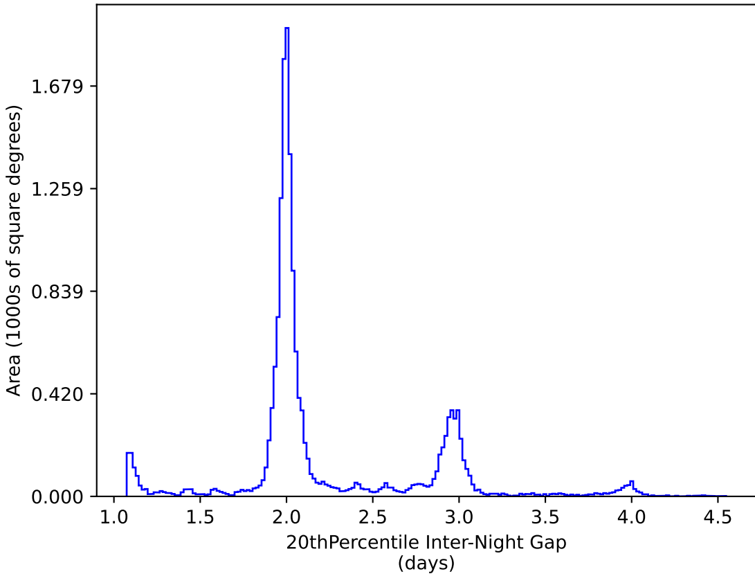
baseline_v3.2_10yrs WFD y band: 20thPercentile Inter-Night Gap
