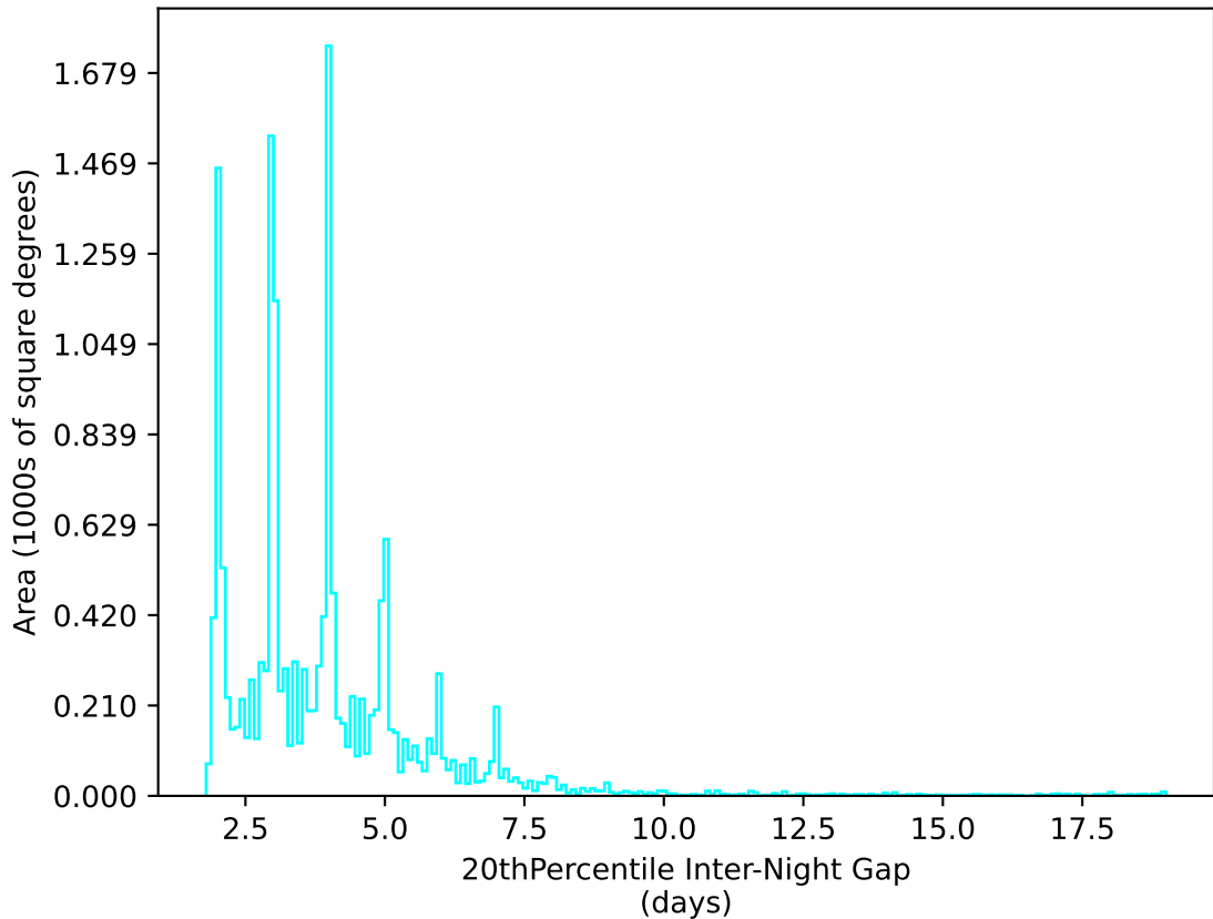
baseline_v3.2_10yrs WFD u band: 20thPercentile Inter-Night Gap
