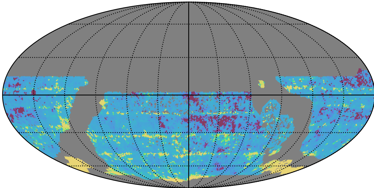
baseline_v3.2_10yrs WFD r band: 20thPercentile Inter-Night Gap
