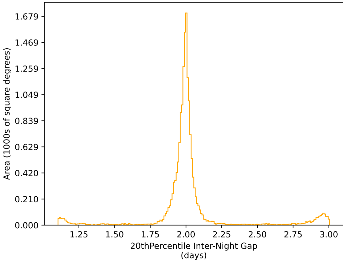
baseline_v3.2_10yrs WFD r band: 20thPercentile Inter-Night Gap
