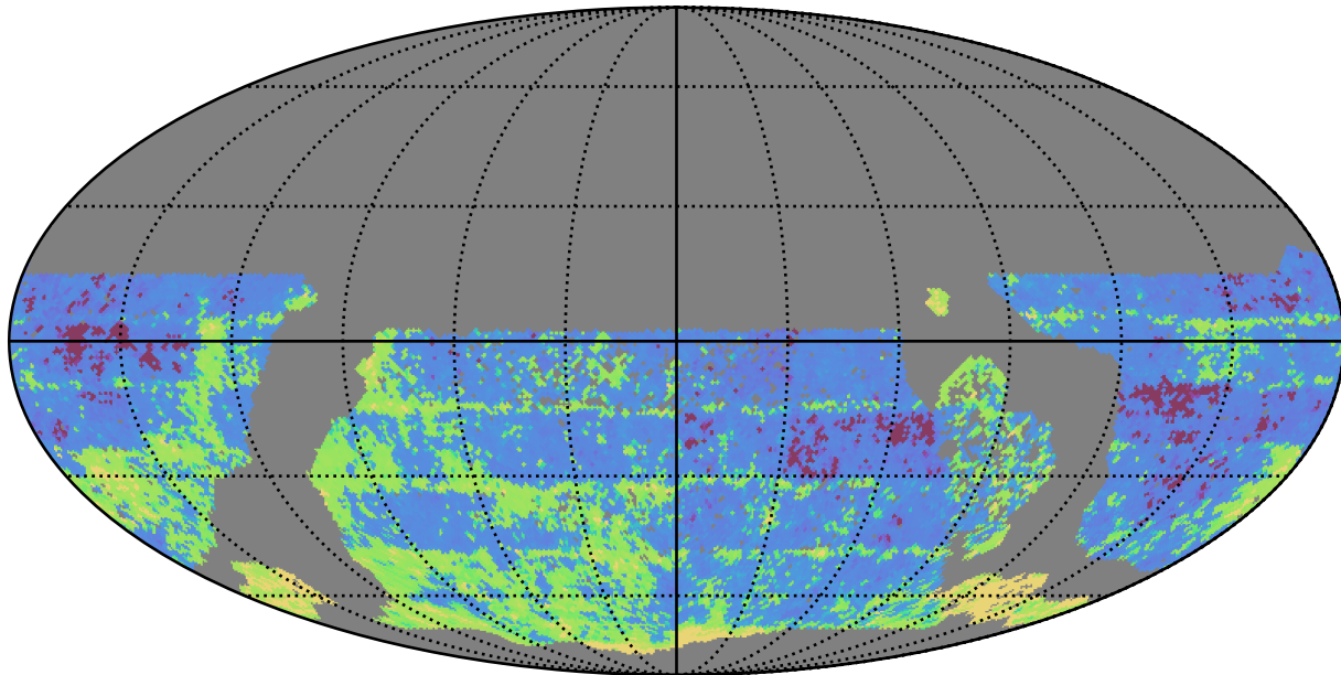
baseline_v3.2_10yrs WFD i band: 20thPercentile Inter-Night Gap
