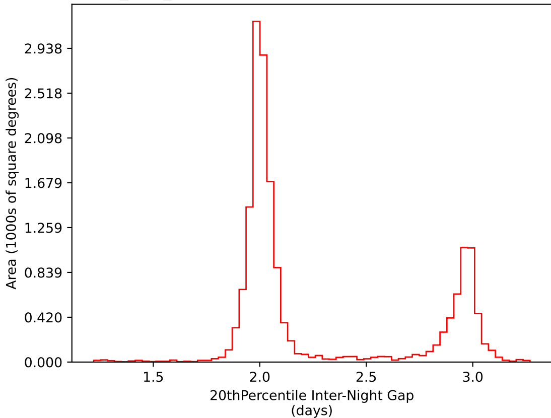
baseline_v3.2_10yrs WFD i band: 20thPercentile Inter-Night Gap
