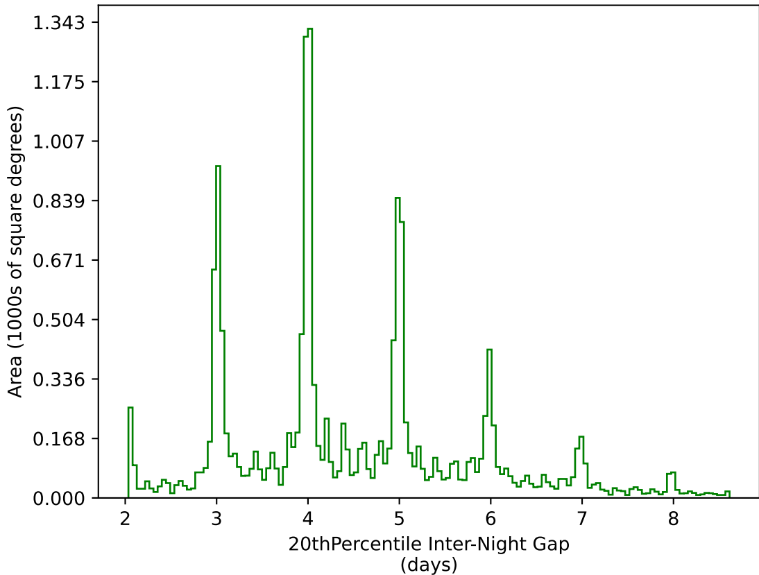
baseline_v3.2_10yrs WFD g band: 20thPercentile Inter-Night Gap
