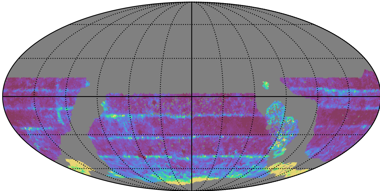
baseline_v3.2_10yrs WFD all bands: 20thPercentile Inter-Night Gap
