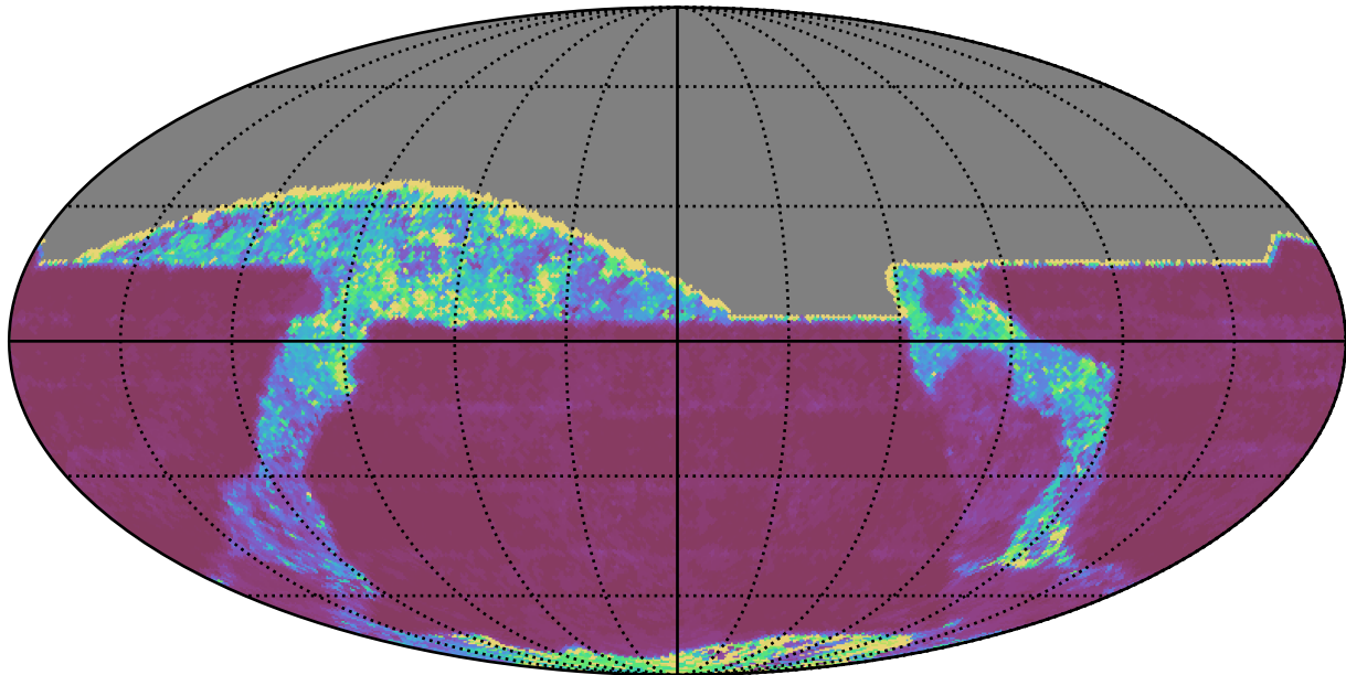
baseline_v3.2_10yrs All sky z band: 20thPercentile Inter-Night Gap
