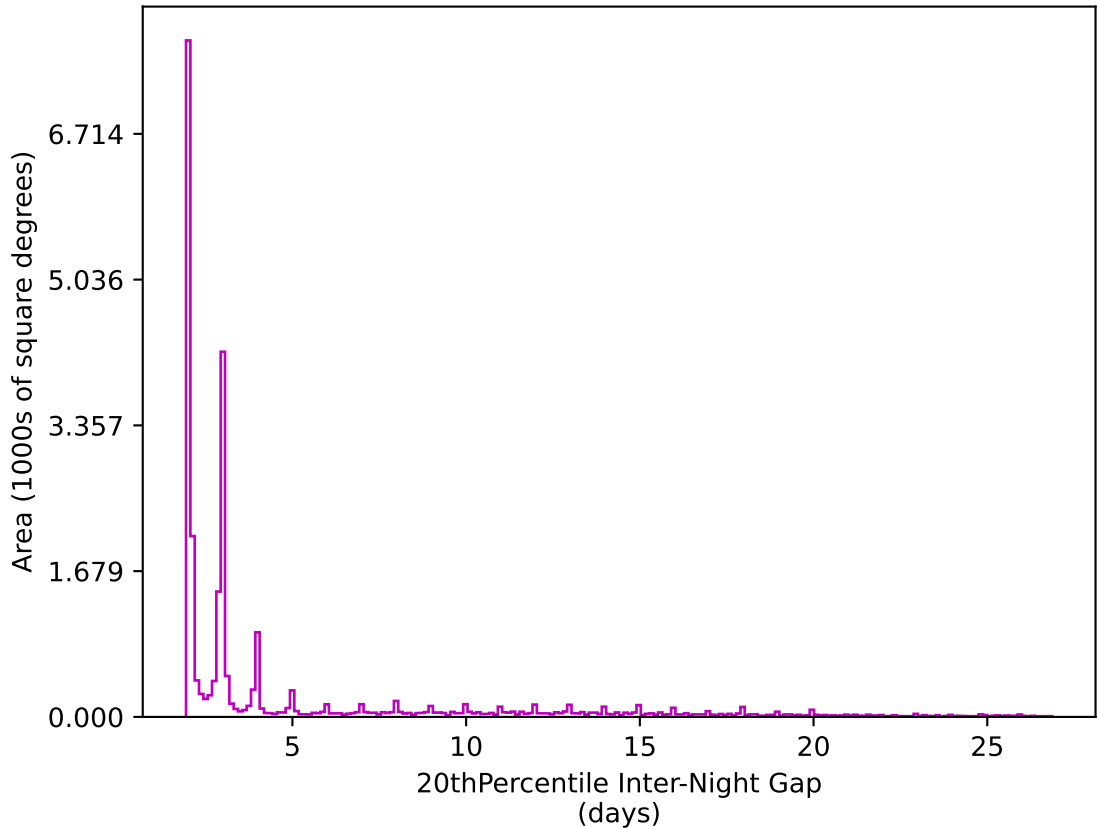
baseline_v3.2_10yrs All sky z band: 20thPercentile Inter-Night Gap
