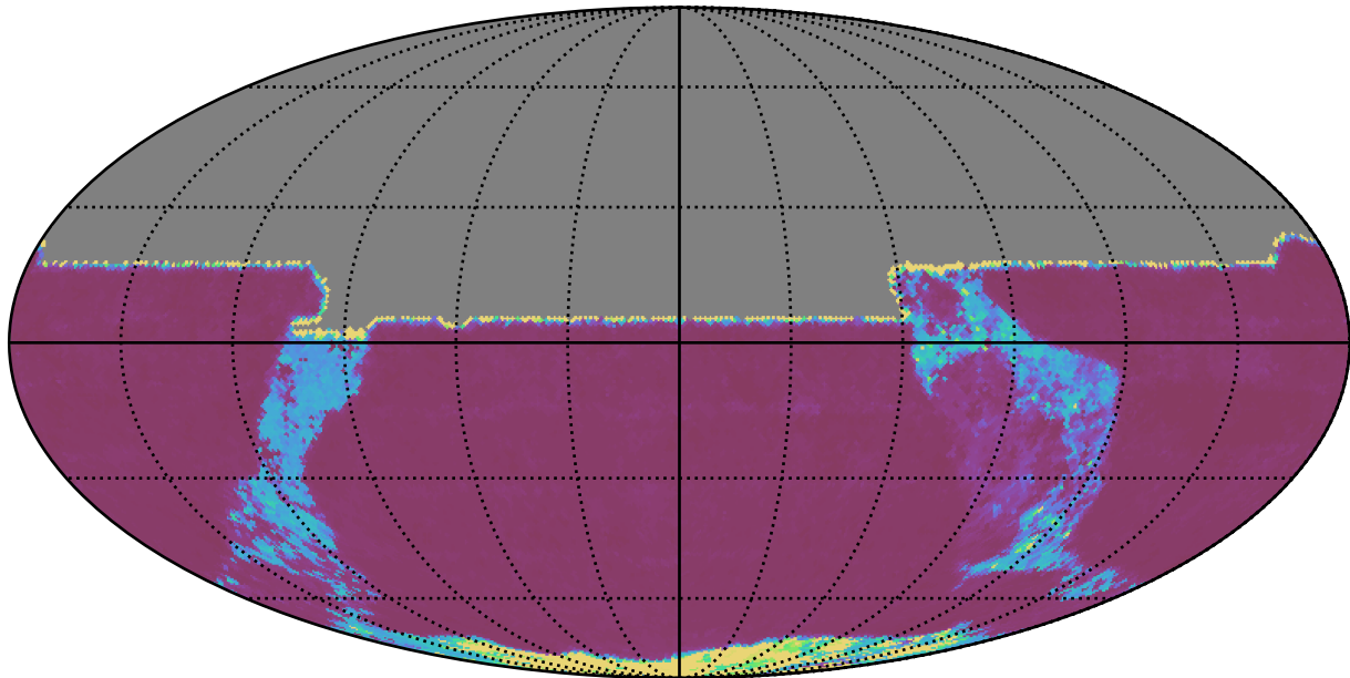
baseline_v3.2_10yrs All sky y band: 20thPercentile Inter-Night Gap
