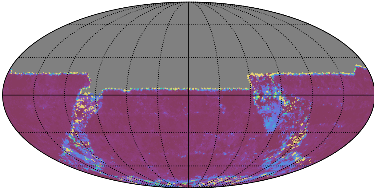
baseline_v3.2_10yrs All sky u band: 20thPercentile Inter-Night Gap
