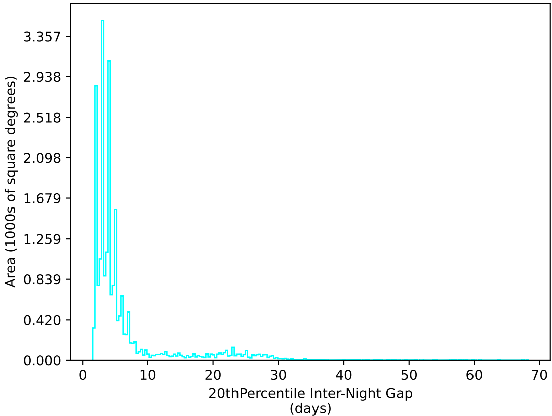
baseline_v3.2_10yrs All sky u band: 20thPercentile Inter-Night Gap
