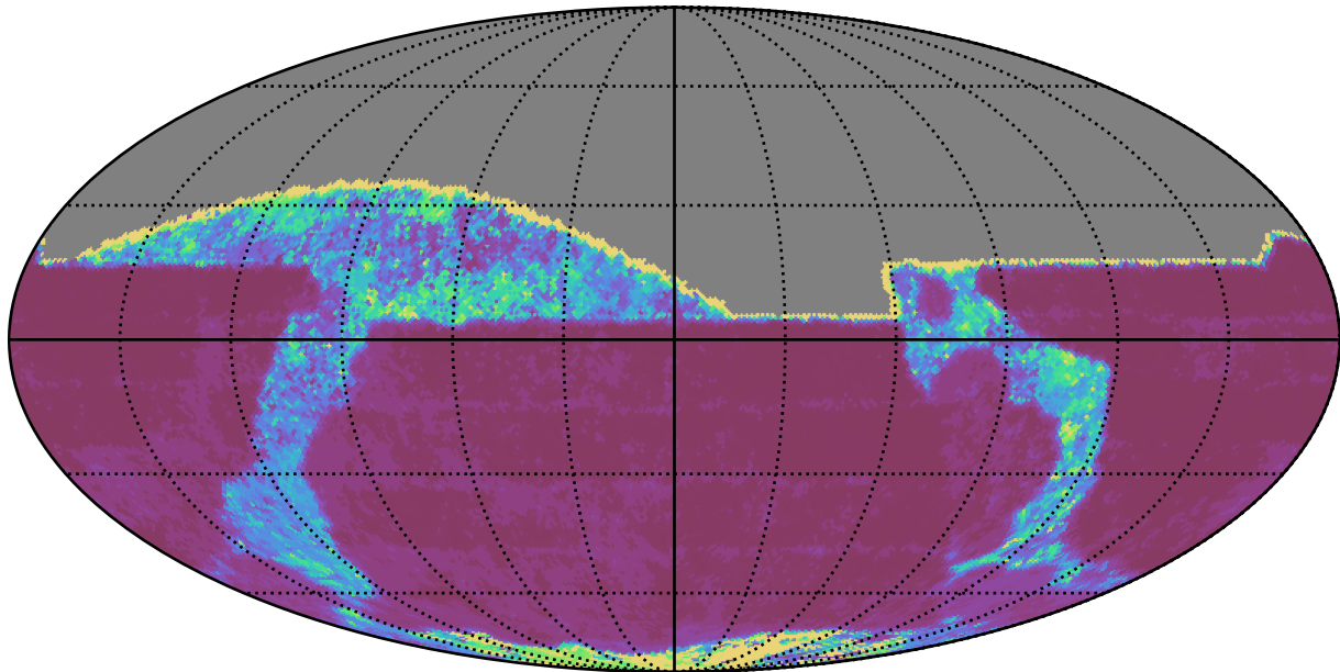
baseline_v3.2_10yrs All sky i band: 20thPercentile Inter-Night Gap
