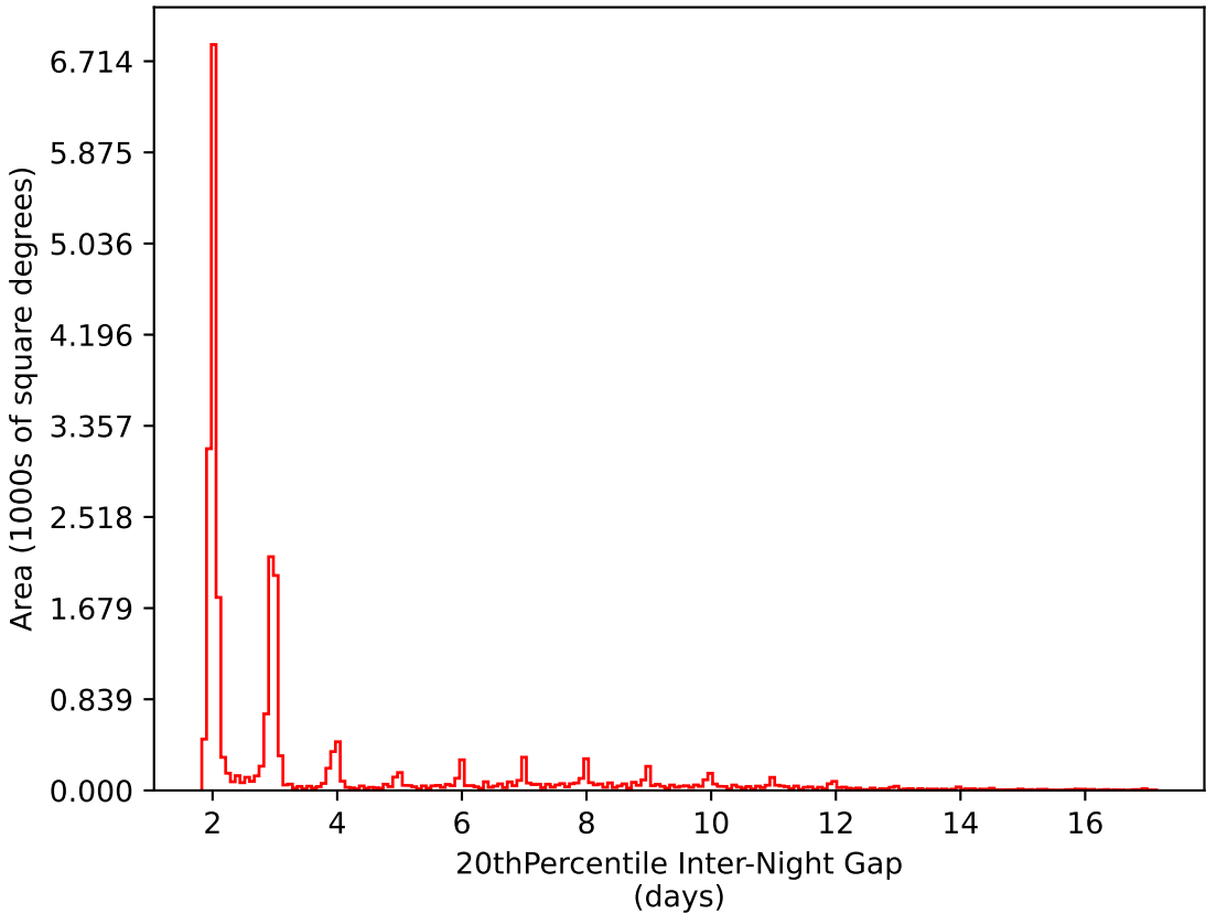
baseline_v3.2_10yrs All sky i band: 20thPercentile Inter-Night Gap
