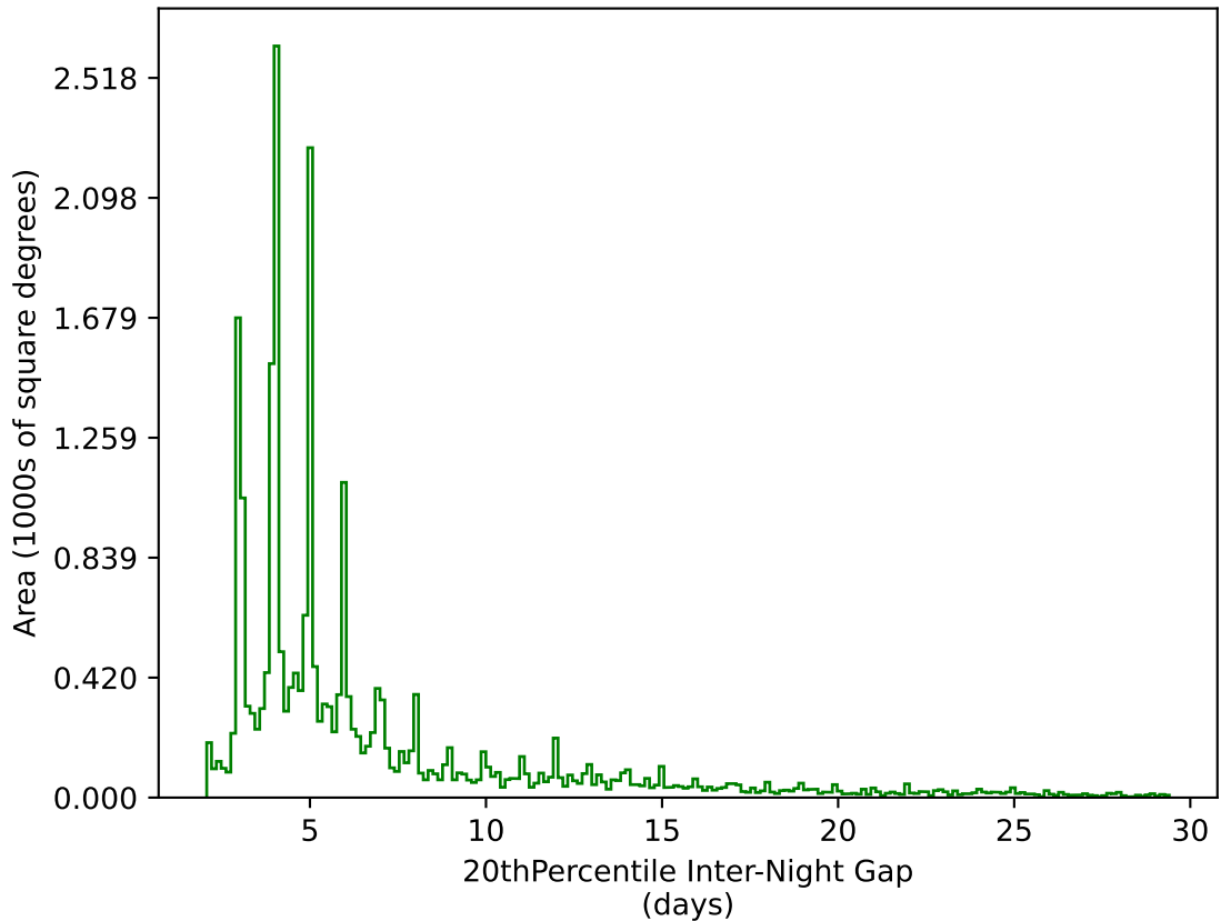
baseline_v3.2_10yrs All sky g band: 20thPercentile Inter-Night Gap
