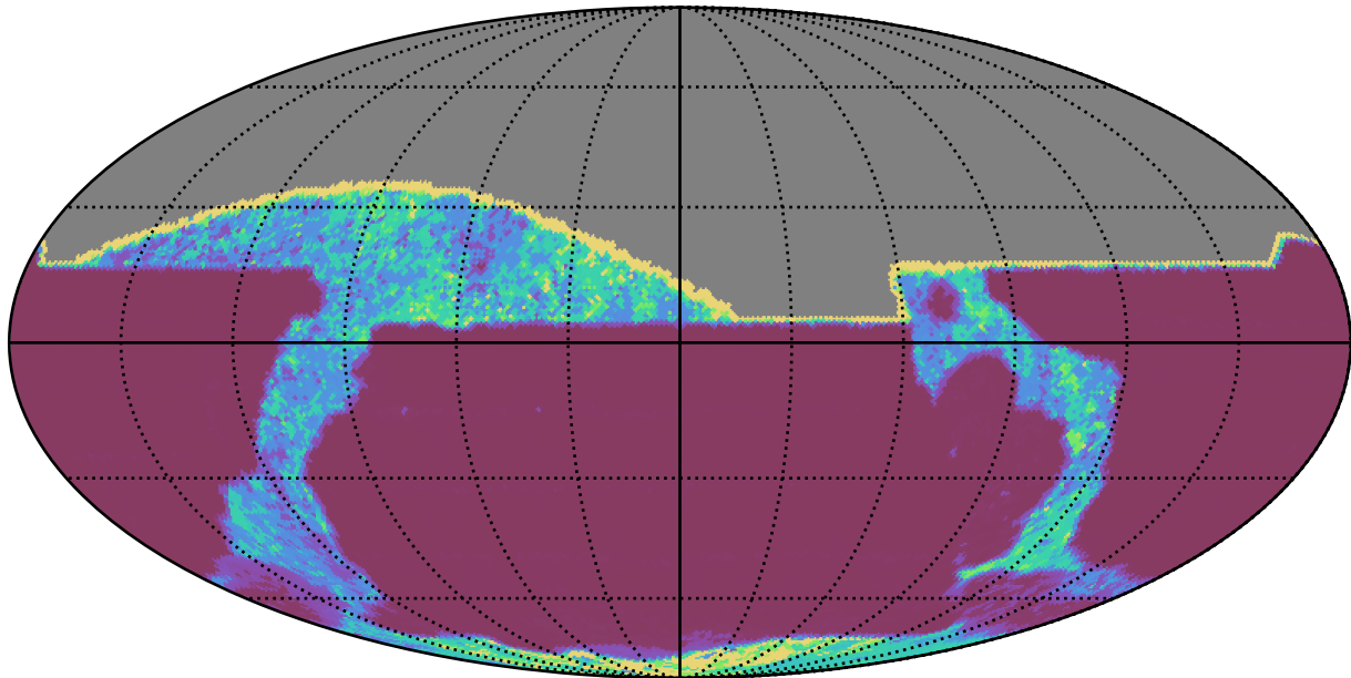
baseline_v3.2_10yrs All sky all bands: 20thPercentile Inter-Night Gap
