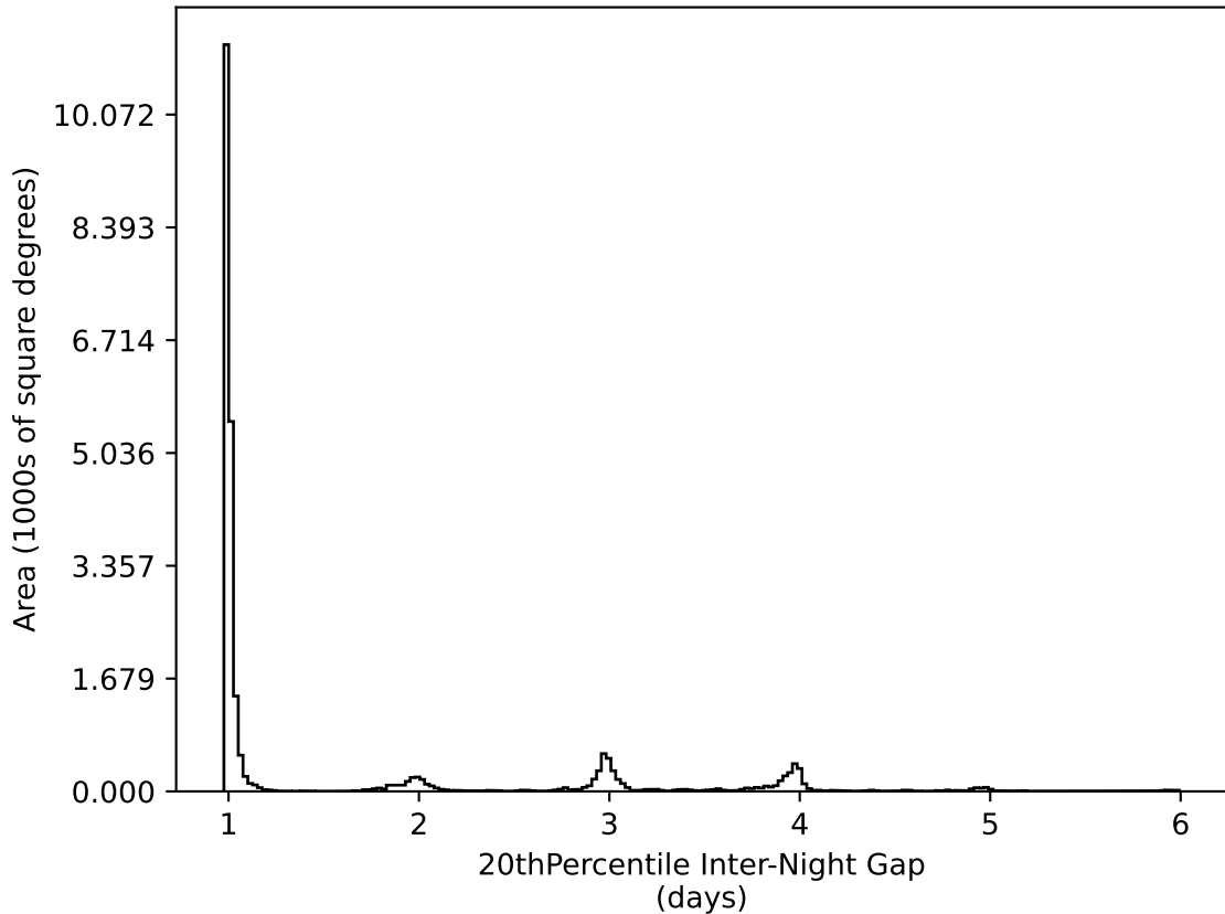
baseline_v3.2_10yrs All sky all bands: 20thPercentile Inter-Night Gap
