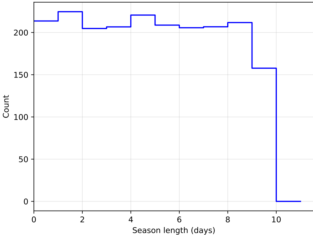
baseline_v3.2_10yrs DD:XMM_LSS all bands: SeasonLength
