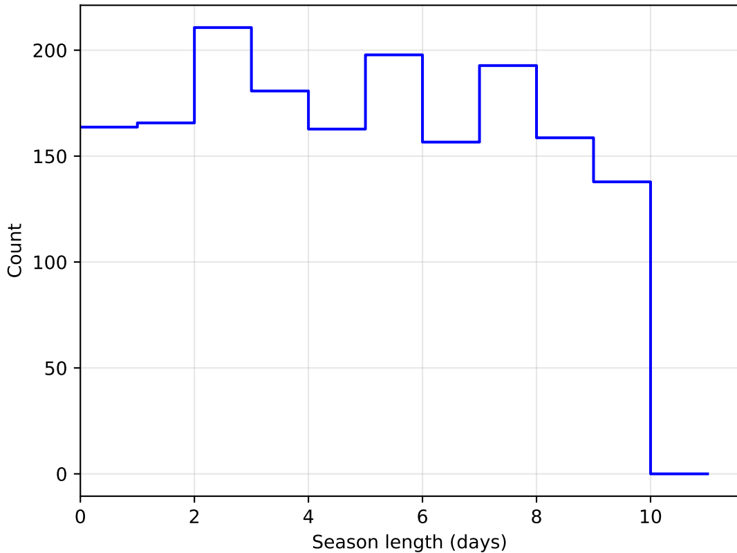
baseline_v3.2_10yrs DD:WFD all bands: SeasonLength
