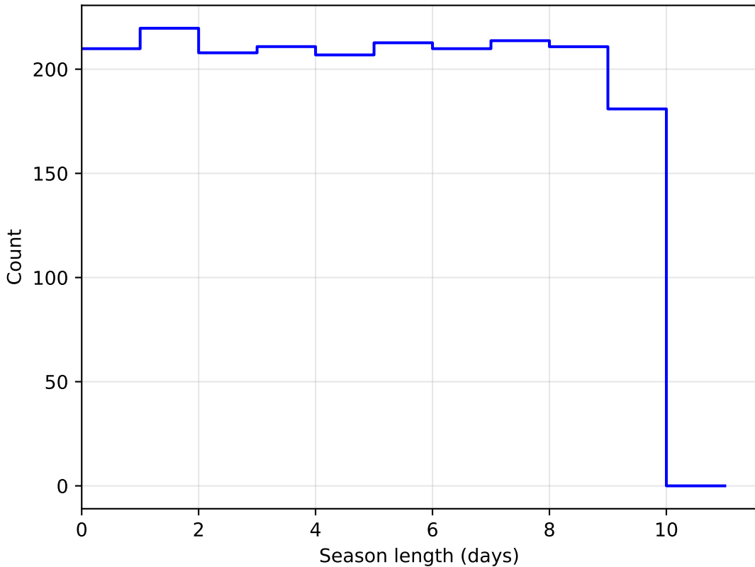
baseline_v3.2_10yrs DD:ELAISS1 all bands: SeasonLength
