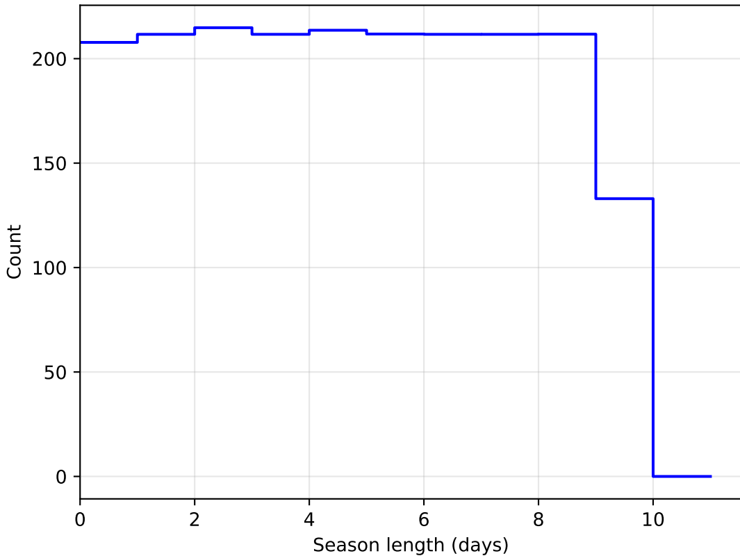
baseline_v3.2_10yrs DD:EDFS all bands: SeasonLength
