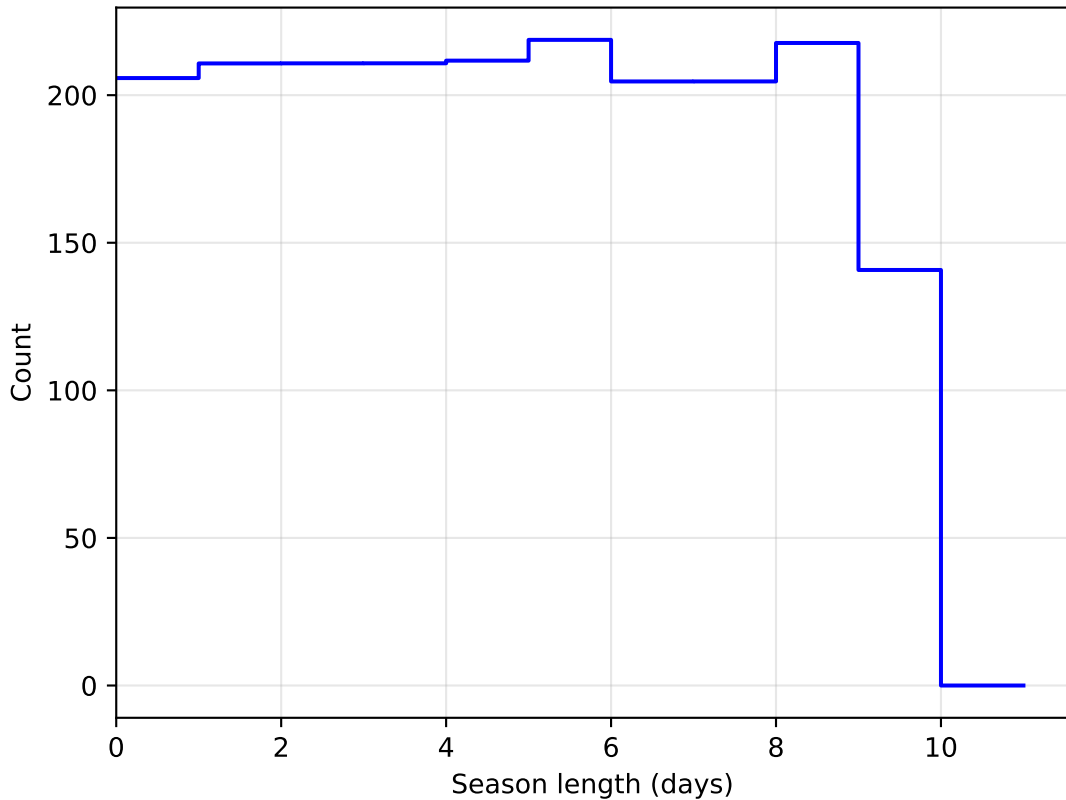
baseline_v3.2_10yrs DD:ECDFS all bands: SeasonLength
