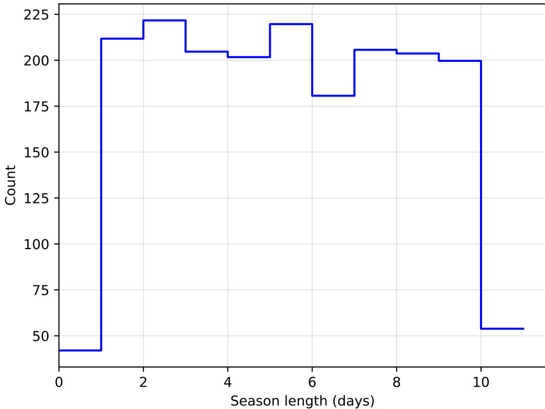
baseline_v3.2_10yrs DD: COSMOS all bands: SeasonLength
