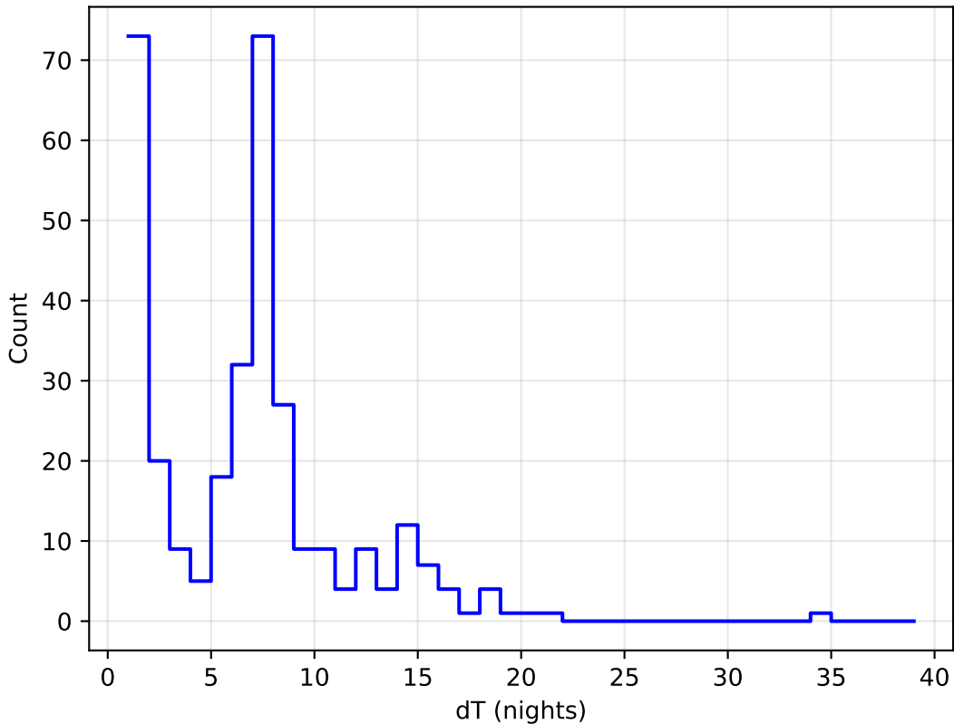
baseline_v3.2_10yrs all bands: DD:XMM_LSS Delta Nights Histogram
