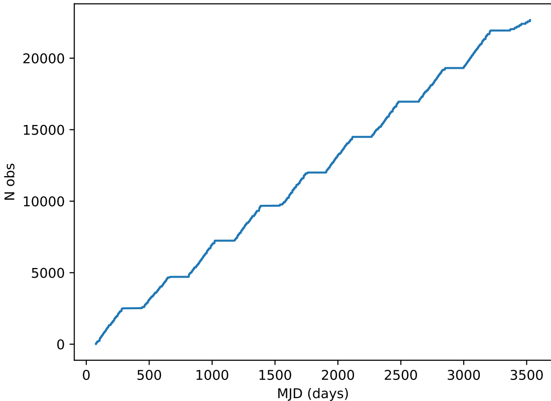
baseline_v3.2_10yrs all bands: DD:XMM_LSS Cumulative NVisits
