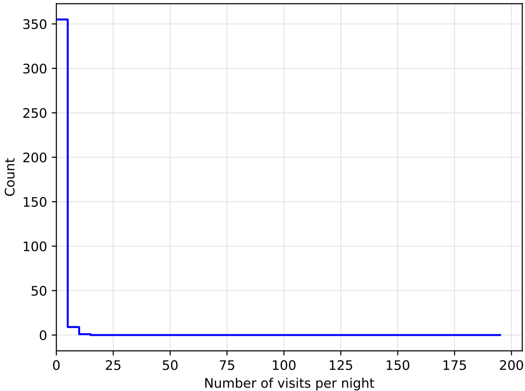
baseline_v3.2_10yrs all bands: DD:WFD NVisitsPerNight
