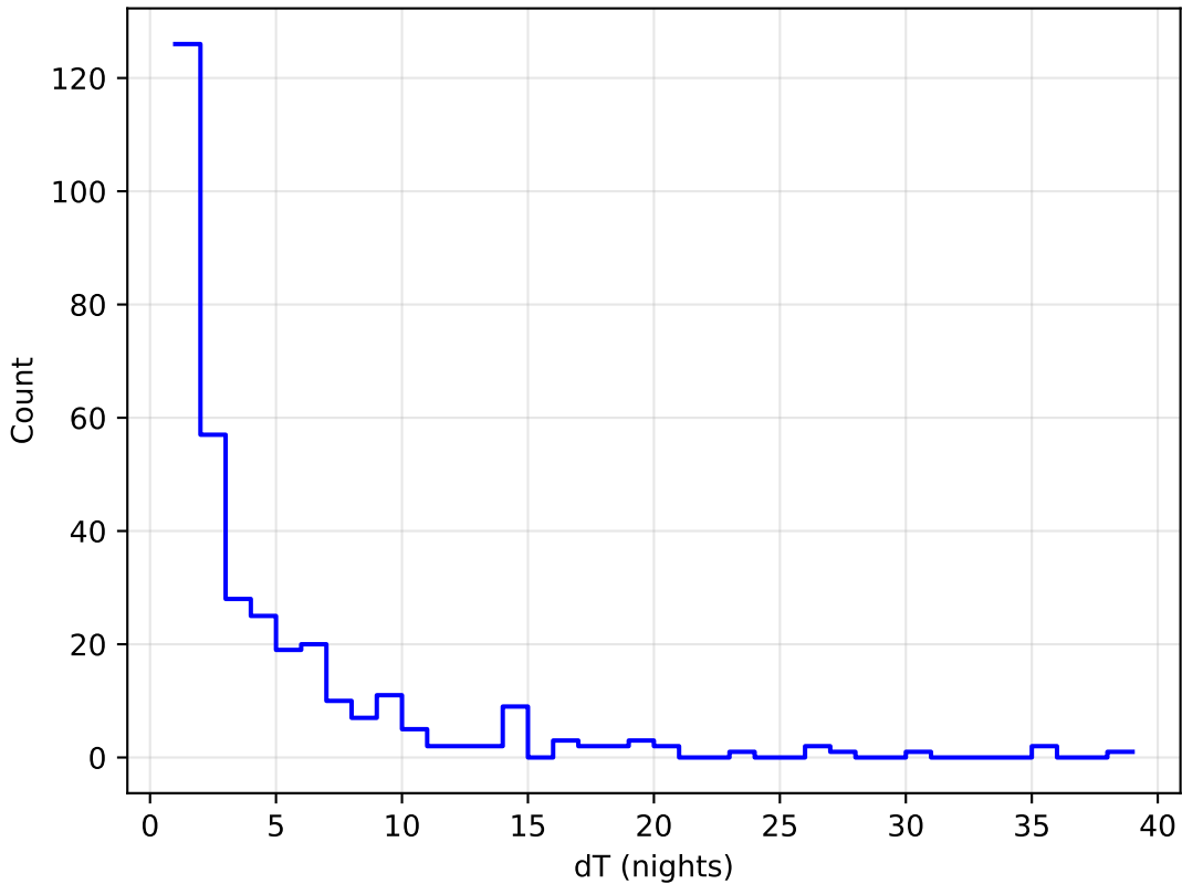
baseline_v3.2_10yrs all bands: DD:WFD Delta Nights Histogram
