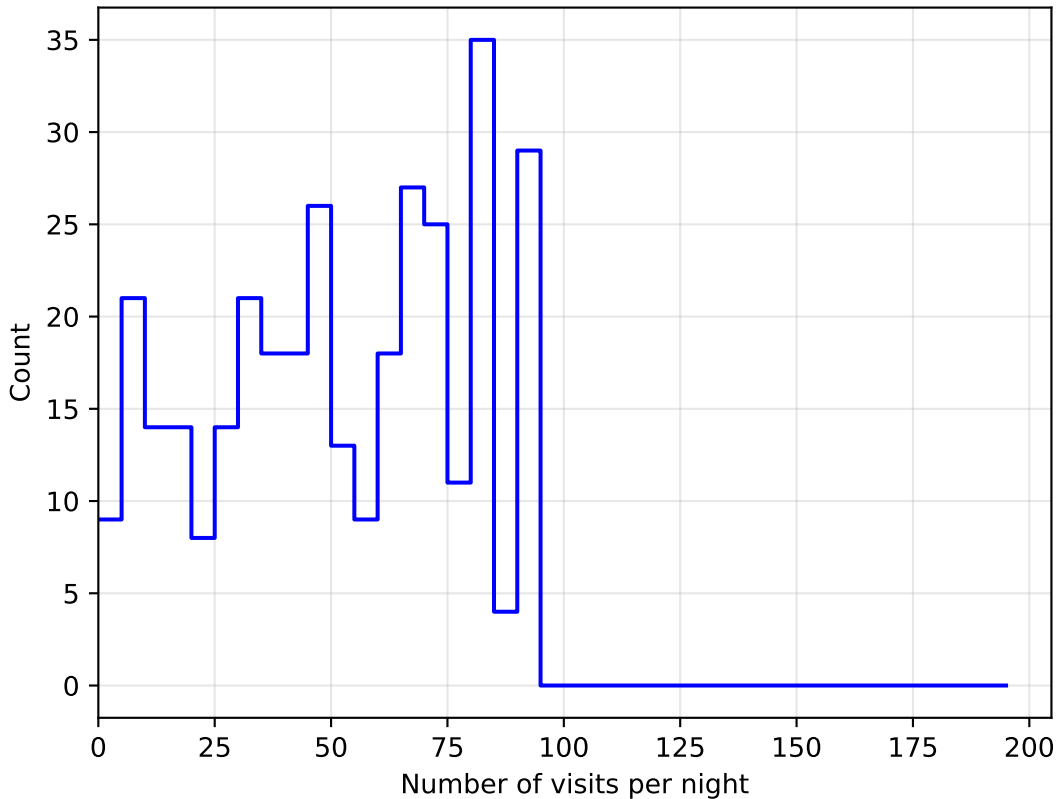
baseline_v3.2_10yrs all bands: DD:EDFS NVisitsPerNight
