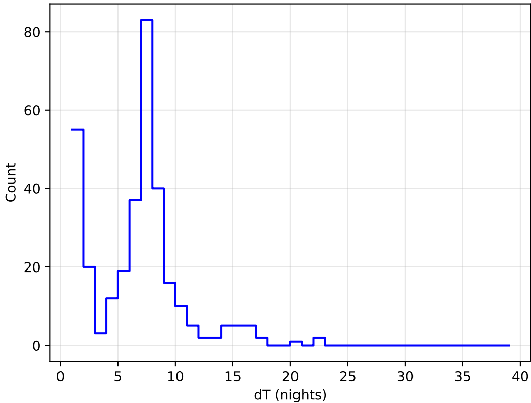
baseline_v3.2_10yrs all bands: DD:EDFS Delta Nights Histogram
