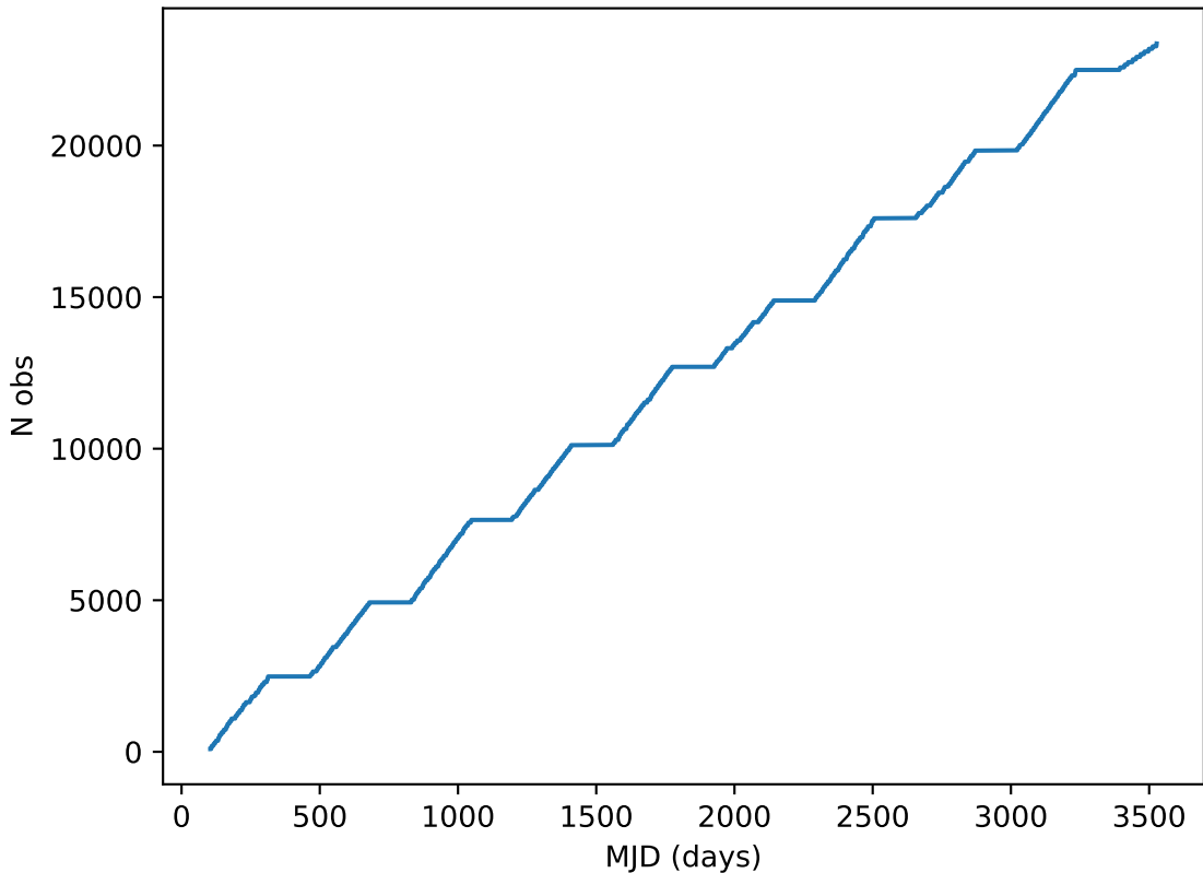
baseline_v3.2_10yrs all bands: DD:EDFS Cumulative NVisits
