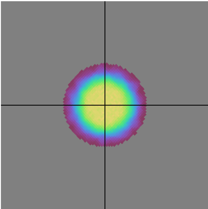
baseline_v3.2_10yrs all bands: DD:ECDFS NVisits
