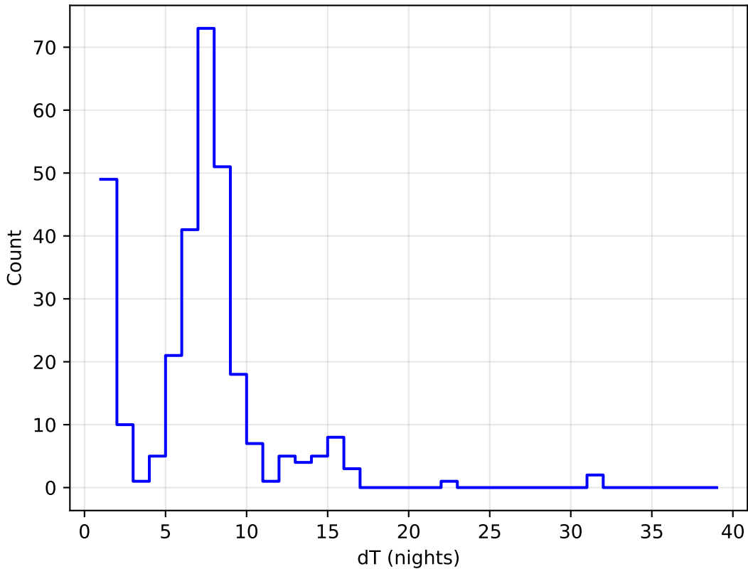
baseline_v3.2_10yrs all bands: DD:ECDFS Delta Nights Histogram
