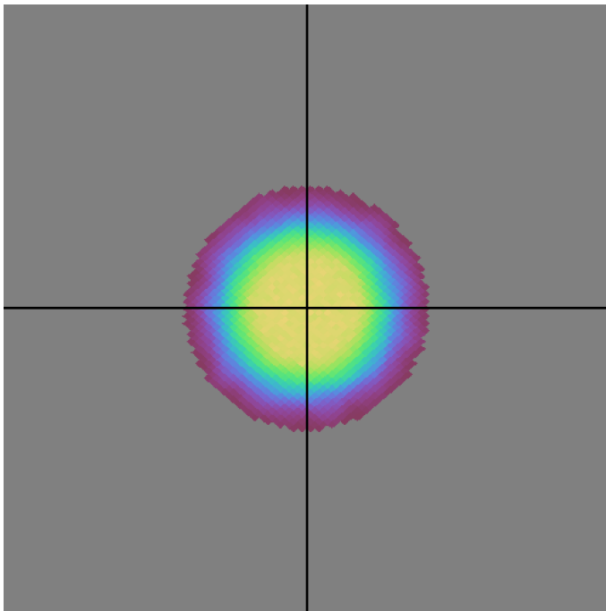
baseline_v3.2_10yrs r band: DD: COSMOS NVisits
