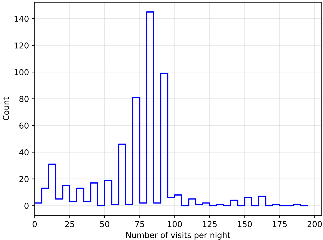
baseline_v3.2_10yrs all bands: DD: COSMOS NVisitsPerNight
