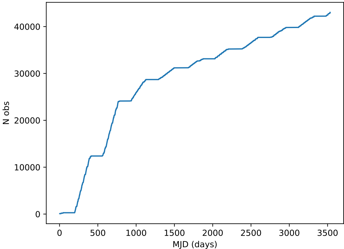
baseline_v3.2_10yrs all bands: DD: COSMOS Cumulative NVisits
