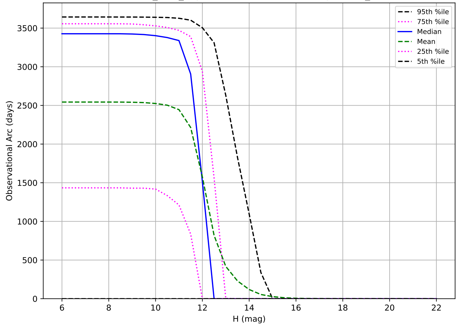
baseline_v3.0_10yrs: Observational Arc Length OCC_r20
