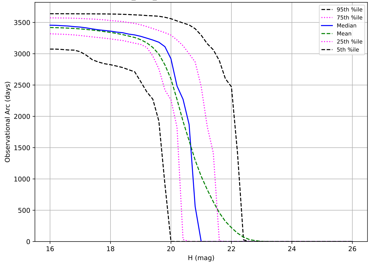
baseline_v3.0_10yrs: Observational Arc Length MBA
