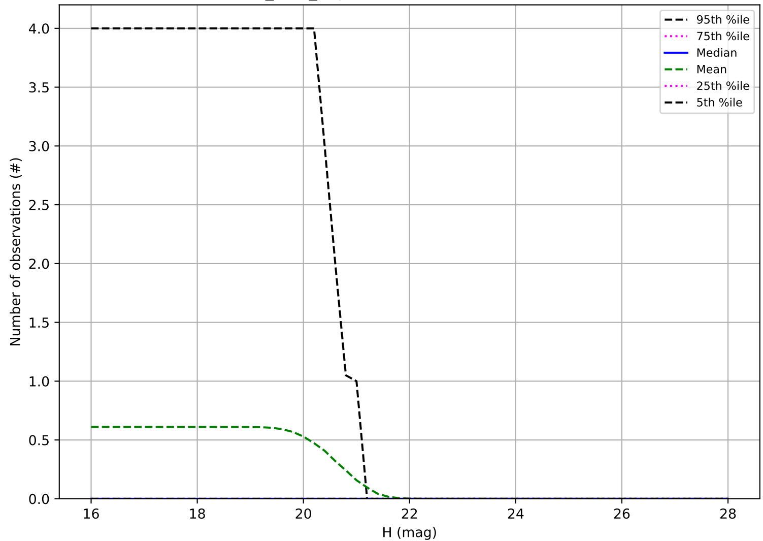
baseline_v3.0_10yrs: Number of observations Vatira
