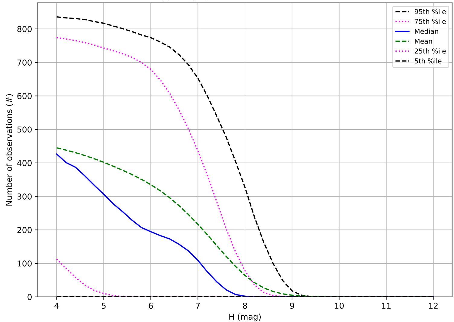
baseline_v3.0_10yrs: Number of observations TNO
