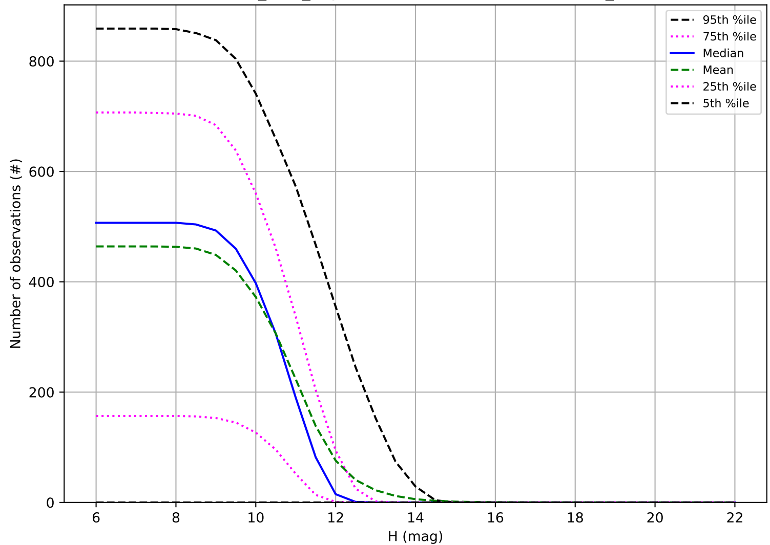
baseline_v3.0_10yrs: Number of observations OCC_r20
